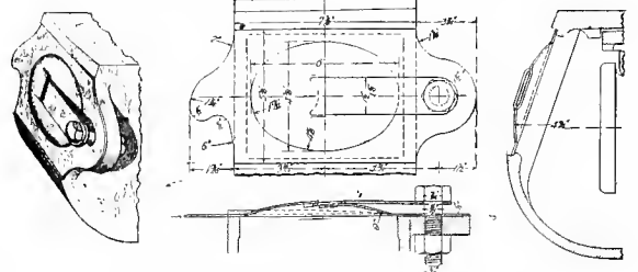
Figs. 5172-5175. THE DREXEL BOX-LID.
